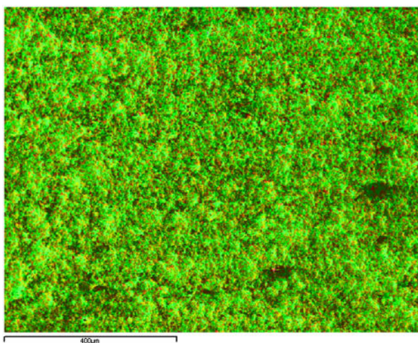
Fig. 1. EDX image of the AgXX® surface: The homogeneous distribution of silver (green) and ruthenium (red) on the surface is shown. The image was generated with a Philips XL 40 SEM with an Oxford EDX microanalysis probe at 125× magnification; working distance from cathode: 10.2 mm. The image was provided by D. Biermann, H. Abrahams (ISF, Dortmund, Germany) and T. Lisowsky (MultiBind biotec GmbH, Cologne, Germany). (For interpretation of the references to color in this figure legend, the reader is referred to the web version of this article.)
