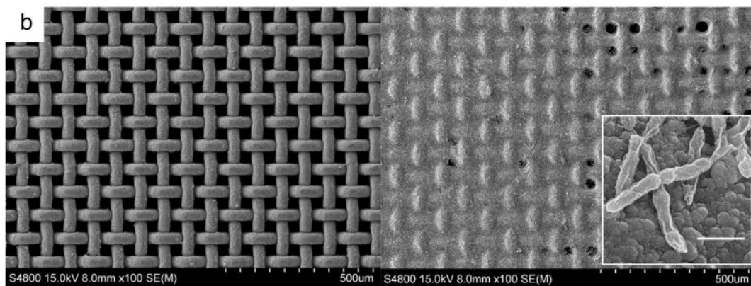
Fig. 6. Effect of AgXX® on growth of Legionella erythra . (a) given as total Hoechst-stainable counts (mean values of 15 counts each per sample). (▲) AgXX®; (■) steel. (b) Inhibition of Legionella surface growth by AgXX®. Left panel, AgXX® mesh after 47 days in CYE medium with Legionella , right panel, steel mesh after 47 days in CYE medium with Legionella . The inset in the right panel shows Legionella cells on the steel mesh (scale bar 1 µm).
