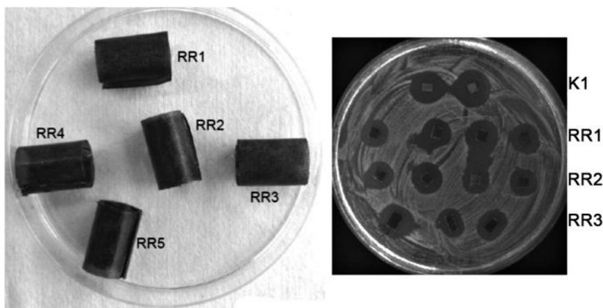
Fig. 8. Long-term activity of AgXX® Left panel: AgXX® Raschig rings (RR 1 to 5) after five years in cooling water for tools in plastics molding. Right panel: RR 1 to RR 3 still showed high antimicrobial activity on E. coli DSM 498 incubated on LB agar for 18 h at 37 °C. K1: AgXX® reference mesh with high antimicrobial activity as positive control. The image was provided by T. Lisowsky, MultiBind biotec GmbH, Cologne, Germany.
