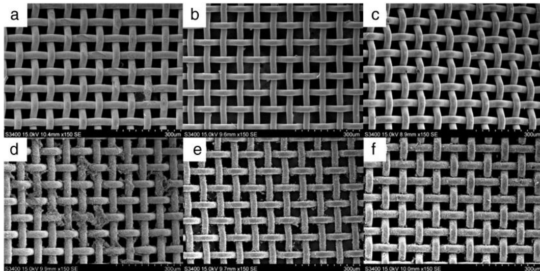
Fig. 5. S. aureus 215642 growth was strongly reduced by AgXX®, reduced by Ag, no effect was observed for uncoated steel. SEM images were taken after incubation in presence of the bacteria for 24 h at 37 °C. Upper panel without bacteria: (a) steel, (b) Ag, (c) AgXX®, lower panel with S. aureus 215642: (d) steel, (e) Ag, (f) AgXX®.
